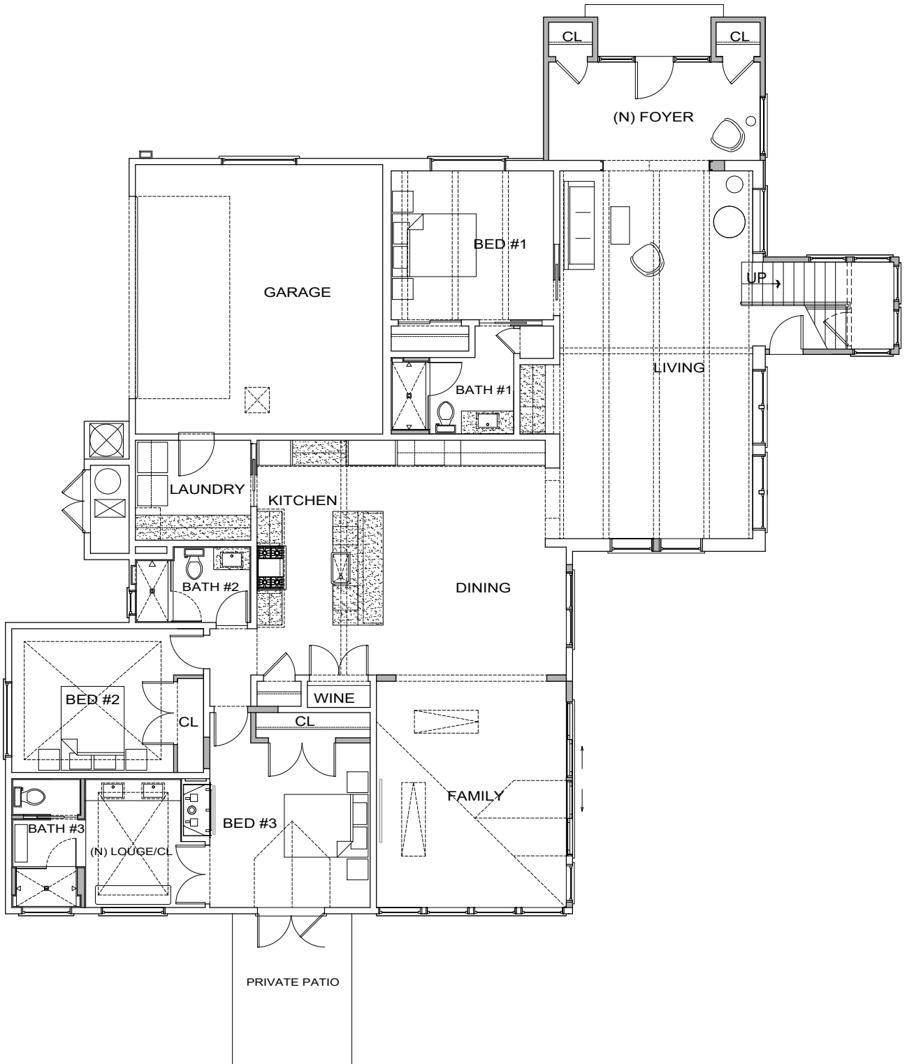
FIRST FLOOR
