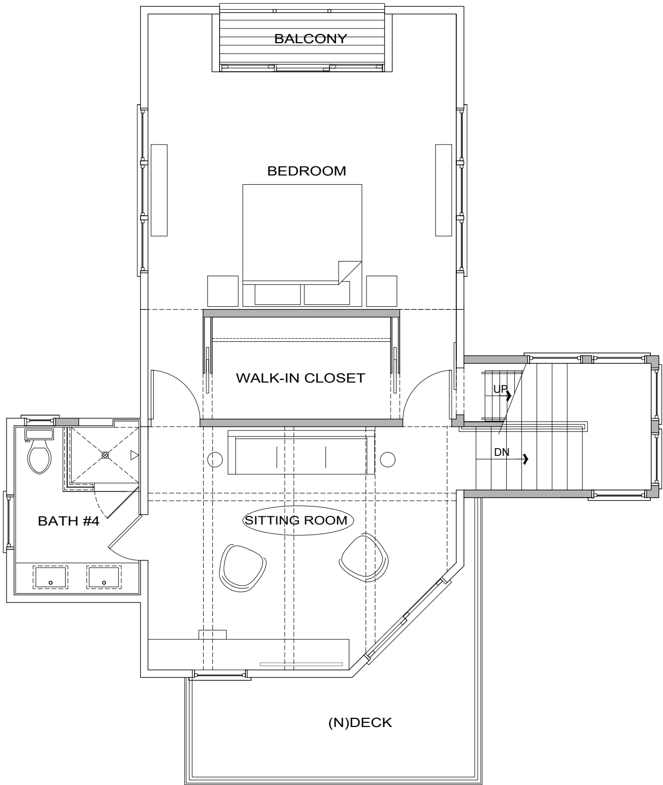
SECOND FLOOR
